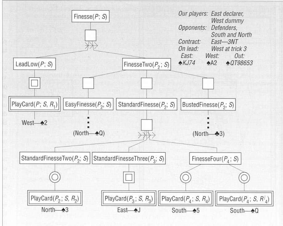
Figure 1. A portion of a finesse method.
