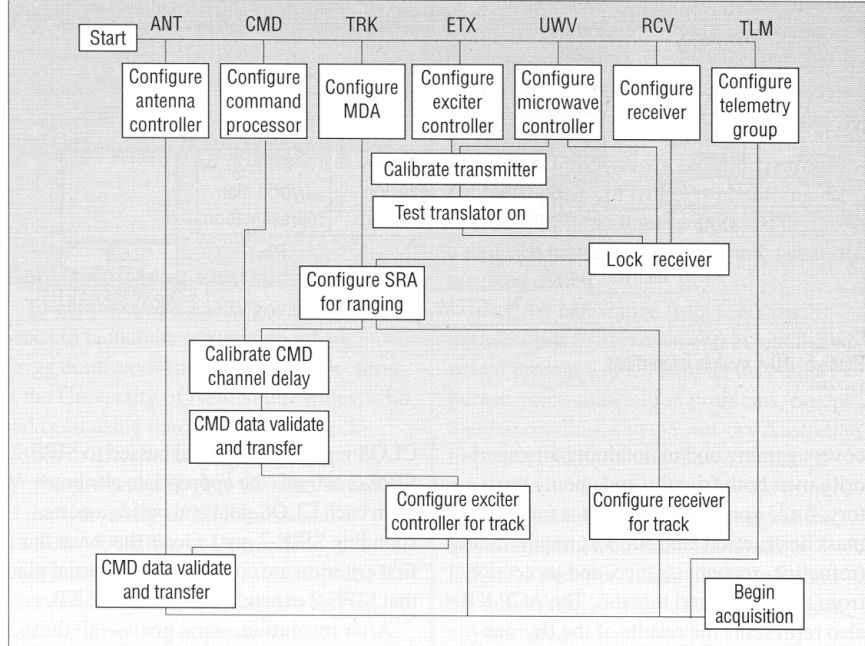
Figure 4. Plan constructed by Dplan for precalibration of a 34-m beam waveguide antenna for telemetry, command, and ranging track.
