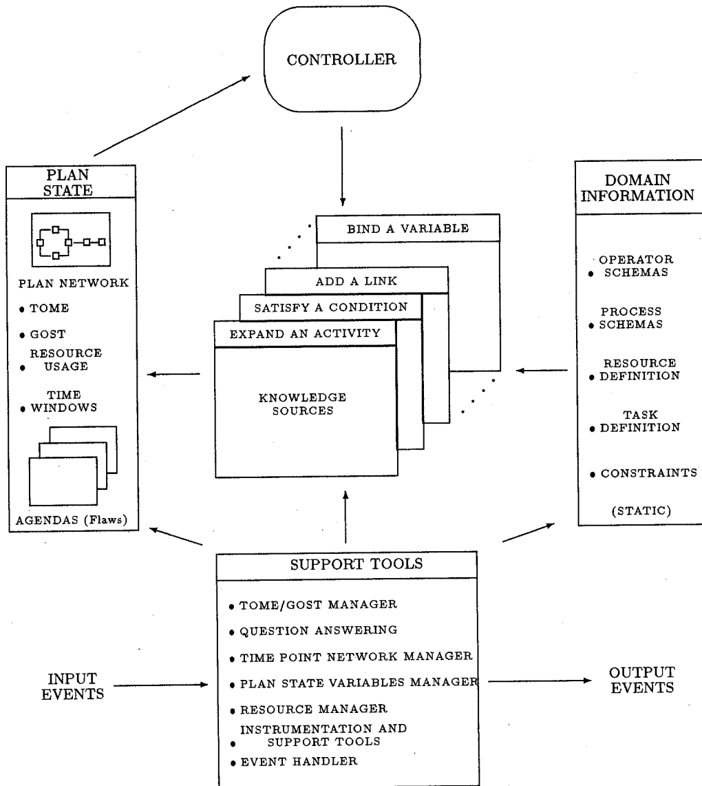
Figure 2: O-Plan2 Architecture
