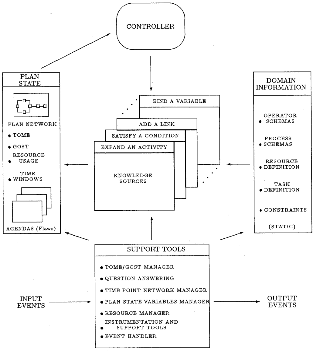
Figure 2: O-Plan2 Architecture
